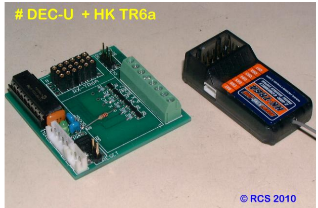
Remove the # EX-LD & binding plug before installing the RX into the # DEC-U. # DEC-U & Tr6a RX shown.
