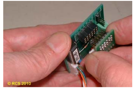
Carefully line up the # DEC-ADAPT ™ pcb with pin #'s 1 - 6 on the # DEC-A and gently press it home onto the pins.
